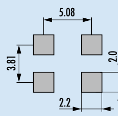
pad layout
